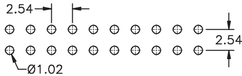
Recommended P.C.B Hole Layout
