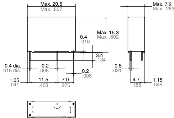
External dimensions
