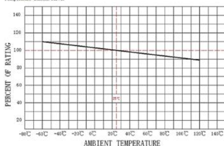
Temperature-Current curve:
