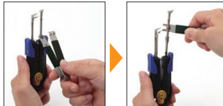
Hook flange with blade removal tool and pry blade upward Blade comes out easily
