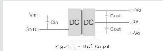
Figure 1 - Dual Output
