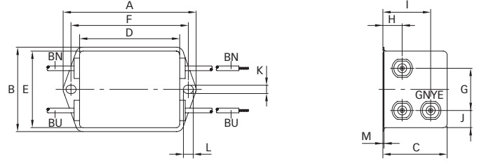
Connection style -07, 10A types
