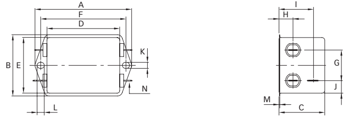
Connection style -06, 10 and 16A types
